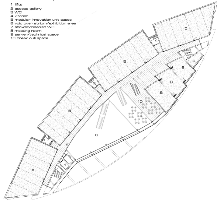
second floor plan 1:250
