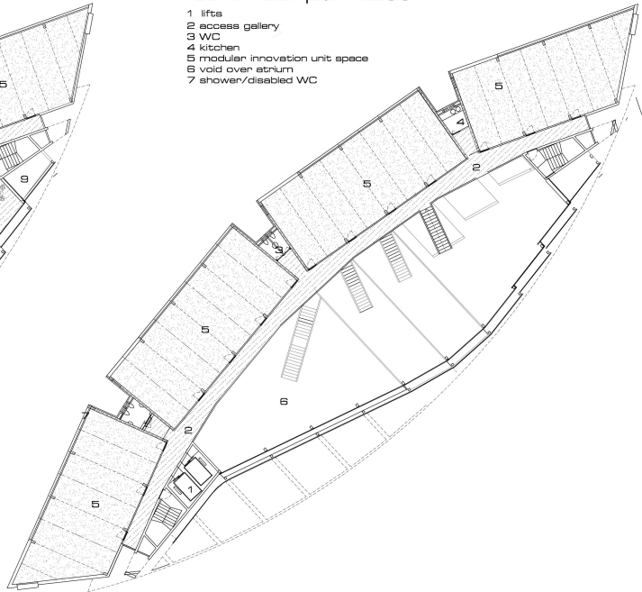
fourth floor plan 1:250
