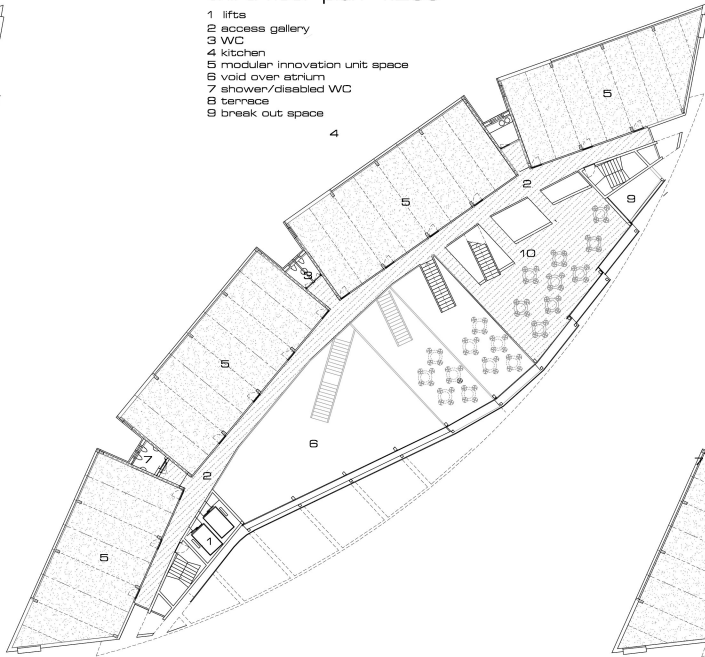
third floor plan 1:250
